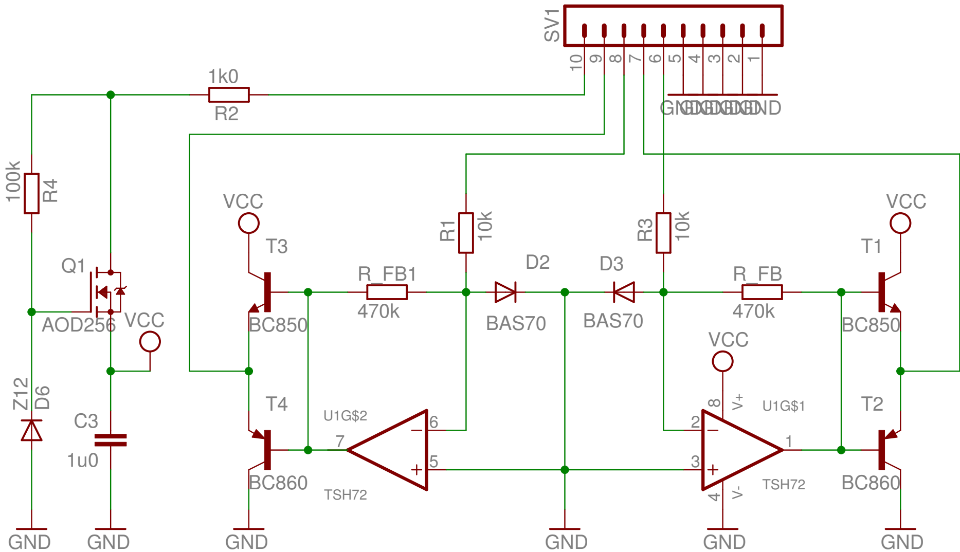
230V-LLC-Converter, sync rect control
